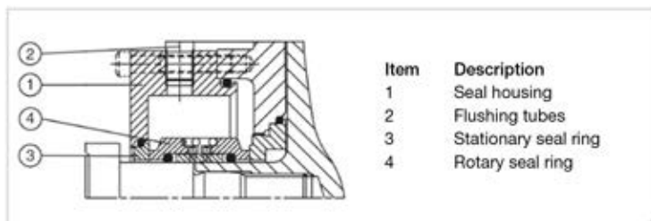
Fig. 6.1j Typical double flushed mechanical seal used in centrifugal pumps
