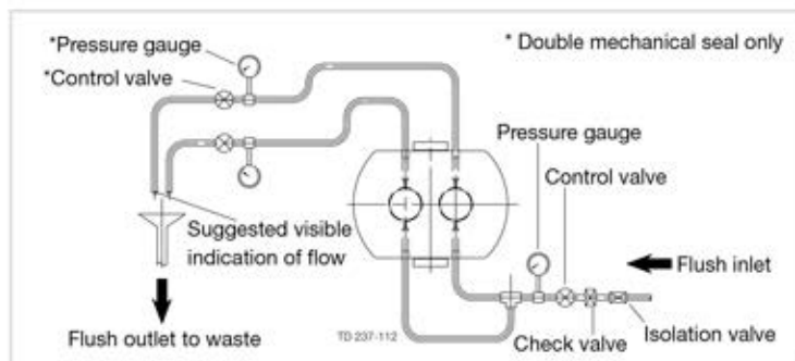
Fig. 6.1k Typical flushing pipework layout for a rotary lobe pump
