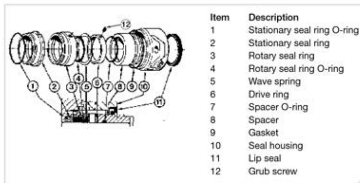
Fig. 6.1g Typical externally mounted single flushed mechanical seal used in rotary lobe pumps
