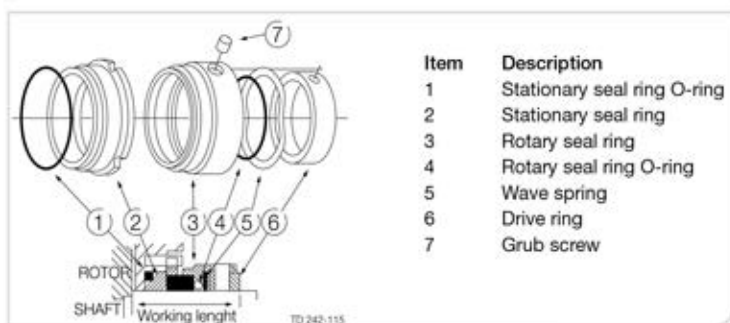
Fig. 6.1a Typical single mechanical seal used in rotary lobe pumps
